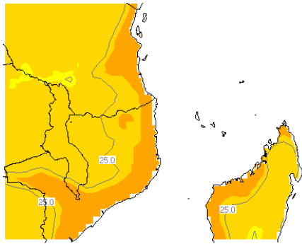
Jan - Monthly Average Mean Temperature
