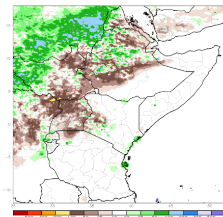
ARC2 1-Month Total Rainfall Anomaly (mm) Period: 01Jul2018 - 31Jul2018
