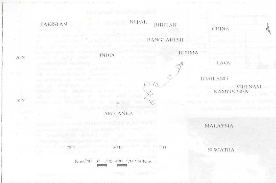
Figure 4: The track of the 01-B storm in the Bay of Bengal from the 11 th to the 19 th is shown. This was a relatively weak storm that achieved the status of a cyclone only on the 14 th of May. By convention, a cyclone has wind speeds of more than 64 knots and a storm between 34 and 64 knots. Data obtained from http://lwf.ncdc.noaa.gov/img/climate/research/2003/may/01b.gif
