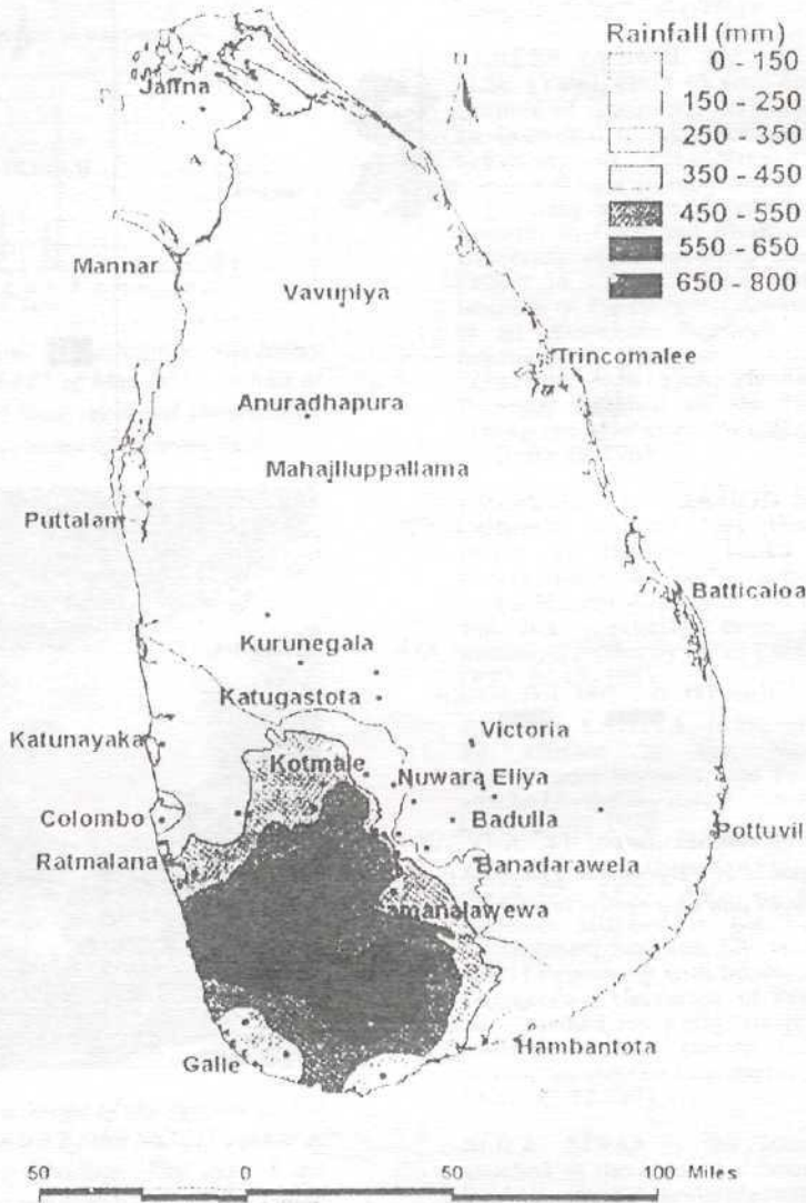
Figure 6: The rainfall during May 2003 is shown and it is heavily concentrated in two areas – one the South-West of Sri Pada (Ratnapura, Kalawana, Badureliya area) and the other South-West of the Gonagala mountain range (Deniyaya). While rainfall is heavily localized, the downstream area will be affected with the resulting floods. Data from Department of Meteorology.
