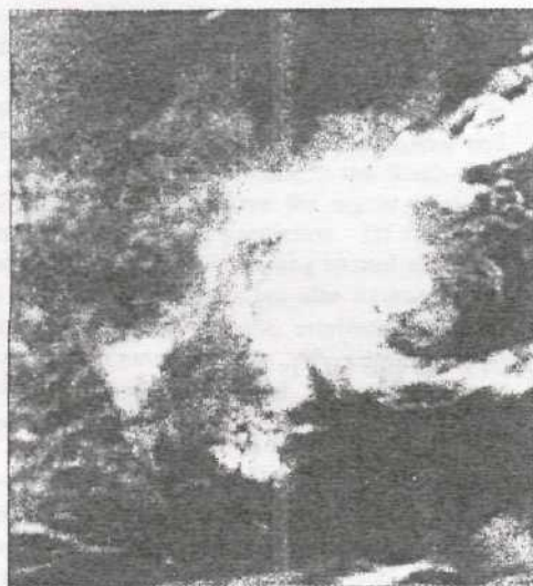
Figure 3: A satellite image of the cyclone on the 14 th of May as recorded by the MODIS sensor of USA's NASA Terra Satellite. The eye of the cyclone is 700 km to the North-East of Sri Lanka and heading away from Sri Lanka. The heaviest deluge in Sri Lanka would come on the 17 th and 18 th of May, when the storm was 1000 km away. Image from ( http://modis.gsfc.nasa.gov/ and http://visibleearth.nasa.gov/ ).
