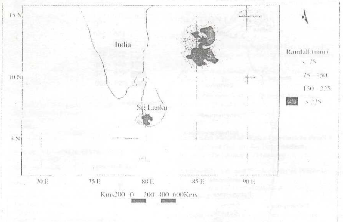
Figure 5. Satellite estimates of rainfall during 15 th to 19 th of May as observed by the Tropical Rainfall Measuring Mission of Japan and USA ( http://trmm.gsfc.nasa.gov/ ) shows that the rainfall was along the track of the cyclone in the Bay of Bengal and also remotely over South-Western Sri Lanka.
