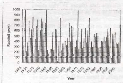
Figure 1: The rainfall observation at Ratnapura, Sri Lanka for May from 1925 to 2003. Data from Department of Meteorology and British Colonial Archives.
