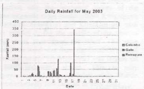
Figure 2: The rainfall at Ratnapura was heavy on the 12 th , 16 th and 17 th of May 2003. A half of the monthly rainfall was recorded on a single day. Data from Department of Meteorology.
