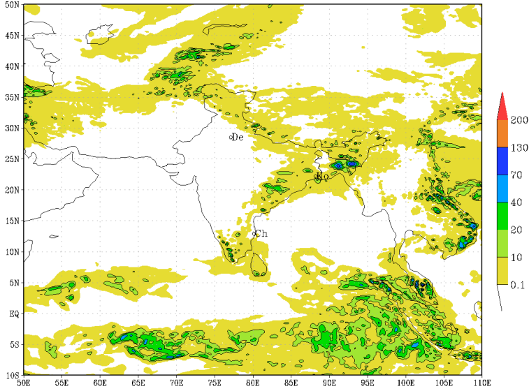
IMD :GFS MODEL(12 Km) RAINFALL (mm) FORECAST (120 HR) based on 00 UTC of 04-04-2020 valid for 03 UTC of 09-04-2020
