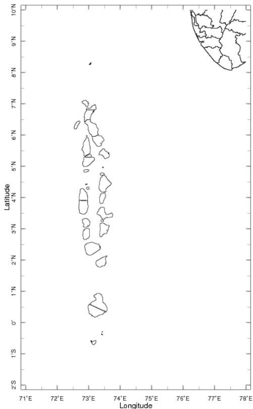
Forecast for 3-8 Apr 2020 Issued 0000 3 Apr 2020
