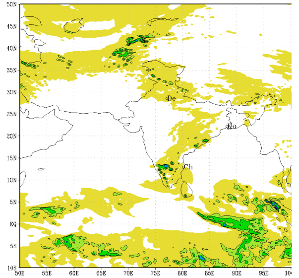
IMD :GFS MODEL(12 Km) RAINFALL (mm) FORECAST based on 00 UTC of 04-04-2020 valid for 03 UTC of 08-04-2020
