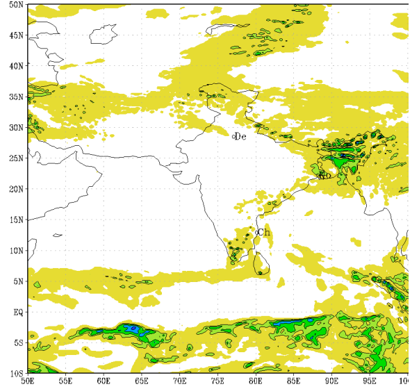
IMD :GFS MODEL(12 Km) RAINFALL (mm) FORECAST based on 00 UTC of 04-04-2020 valid for 03 UTC of 10-04-2020
