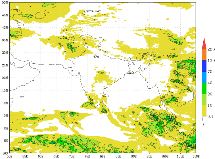
IMD :GFS MODEL(12 Km) RAINFALL (mm) FORECAST (72 HR) based on 00 UTC of 04-04-2020 valid for 03 UTC of 07-04-2020
