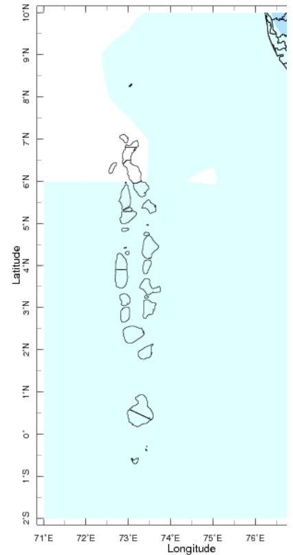
Forecast for 3-8 Apr 2020 Issued 0000 3 Apr 2020
