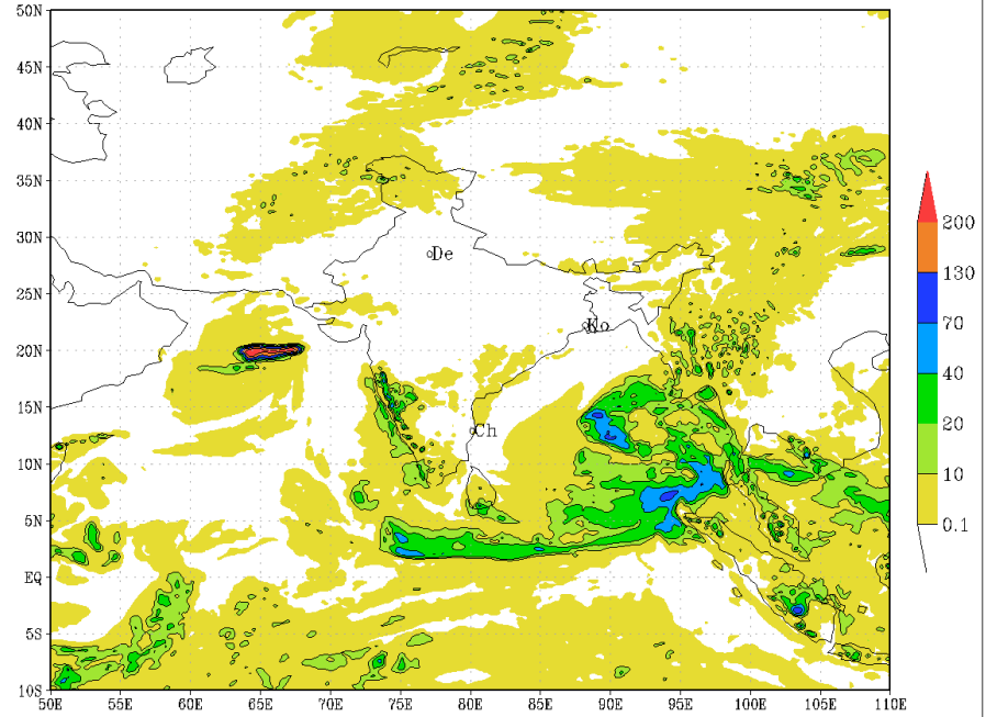
IMD :GFS MODEL(12 Km) RAINFALL (mm) FORECAST (48 HR) based on 00 UTC of 04-11-2019 valid for 03 UTC of 06-11-2019
