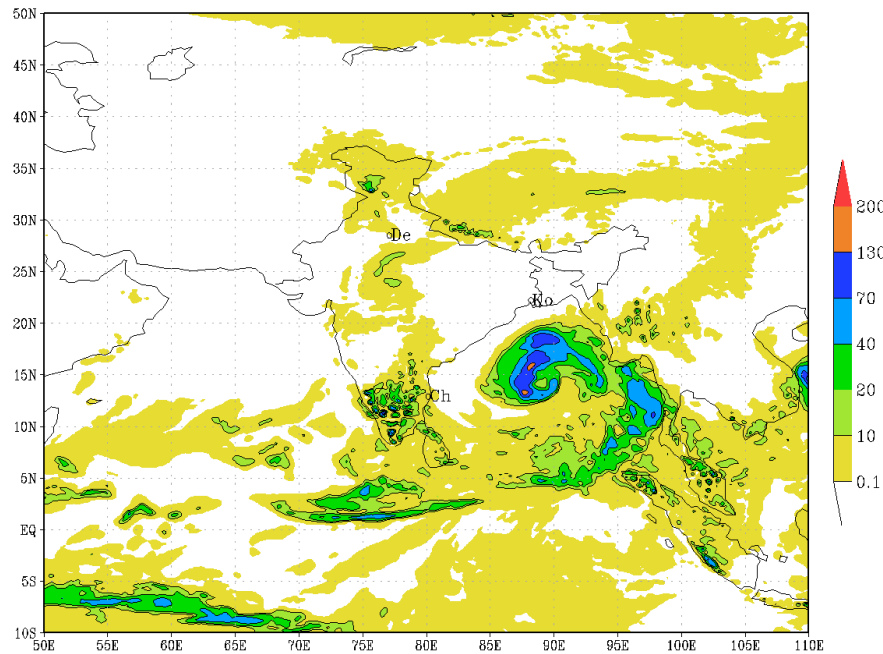
IMD :GFS MODEL(12 Km) RAINFALL (mm) FORECAST (120 HR) based on 00 UTC of 04-11-2019 valid for 03 UTC of 09-11-2019
