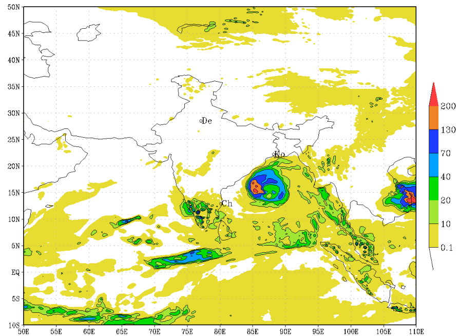
IMD :GFS MODEL(12 Km) RAINFALL (mm) FORECAST (144 HR) based on 00 UTC of 04-11-2019 valid for 03 UTC of 10-11-2019
