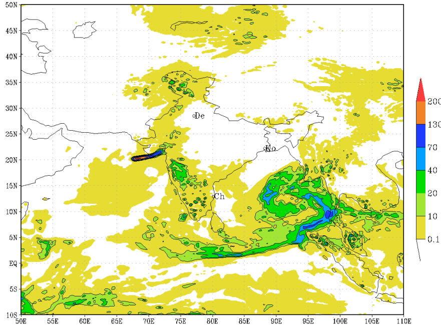
IMD :GFS MODEL(12 Km) RAINFALL (mm) FORECAST (72 HR) based on 00 UTC of 04-11-2019 valid for 03 UTC of 07-11-2019
