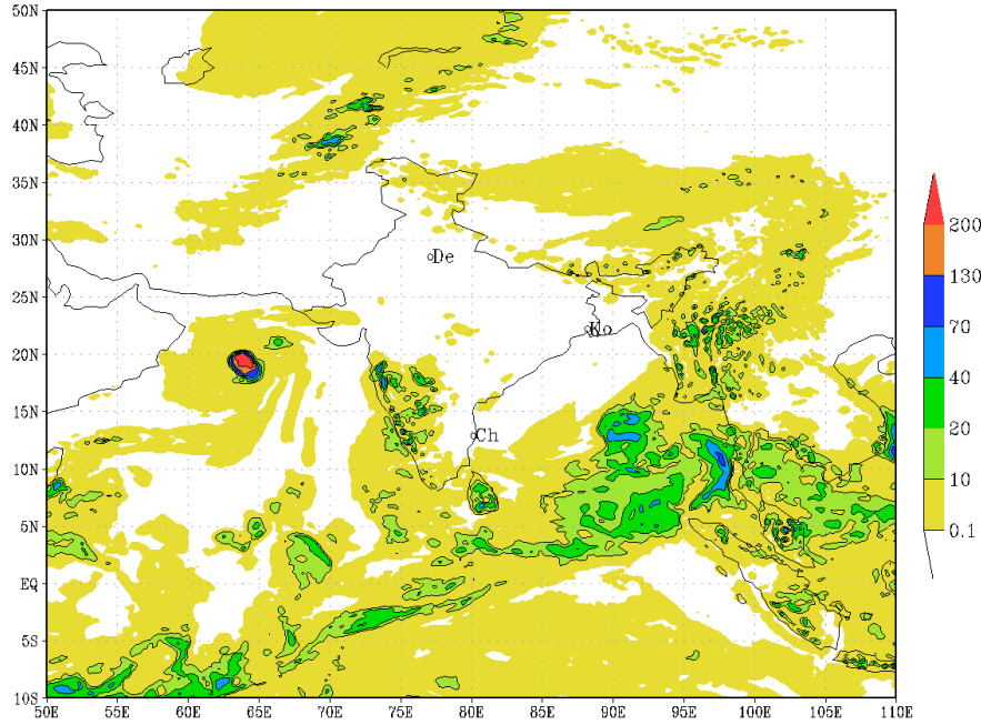
IMD :GFS MODEL(12 Km) RAINFALL (mm) FORECAST (24 HR) based on 00 UTC of 04-11-2019 valid for 03 UTC of 05-11-2019
