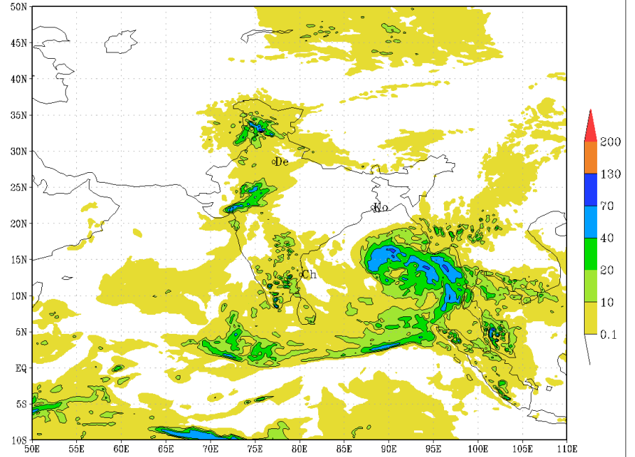
IMD :GFS MODEL(12 Km) RAINFALL (mm) FORECAST (96 HR) based on 00 UTC of 04-11-2019 valid for 03 UTC of 08-11-2019
