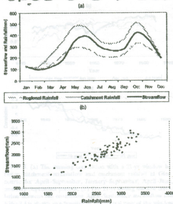
FIG. 3. (a) The climatology of western hills region rainfall, Green-course catchment rainfall, and streamflow for the period 1925-95. (b) Scatterplots of the catchment streamflow vs rainfall for the April-September season.
