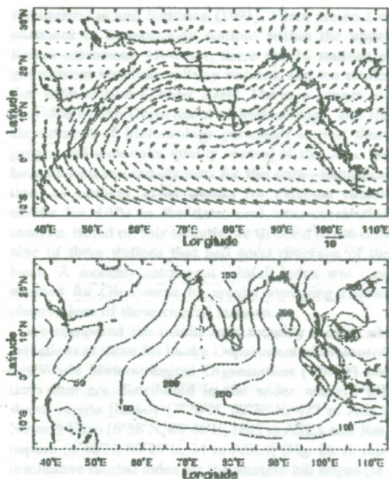
FIG. 1. (a) The mean low-level wind field at 925 mb from April to September for 1958–2002 ( m s^{-1} ). Data obtained from NCEP–NCAR reanalysis (Kistler et al. 2001). (b) The mean monthly rainfall during April–September for 1979–2004 ( mm month^{-1} ). Data obtained from the CAMS_GPI dataset (Janowiak and Xie 1999).
