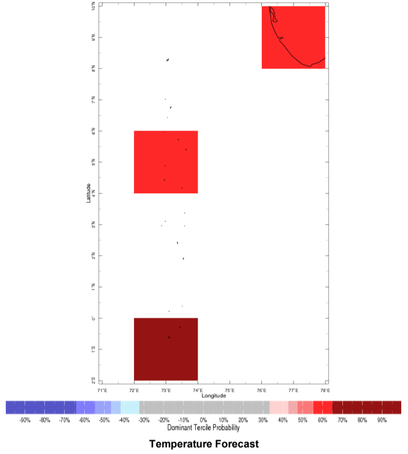
Mar-May 2015 IRI Seasonal Temperature Forecast issued Feb 2015
