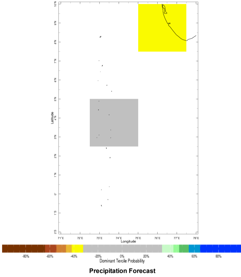
Mar-May 2015 IRI Seasonal Precipitation Forecast issued Feb 2015
