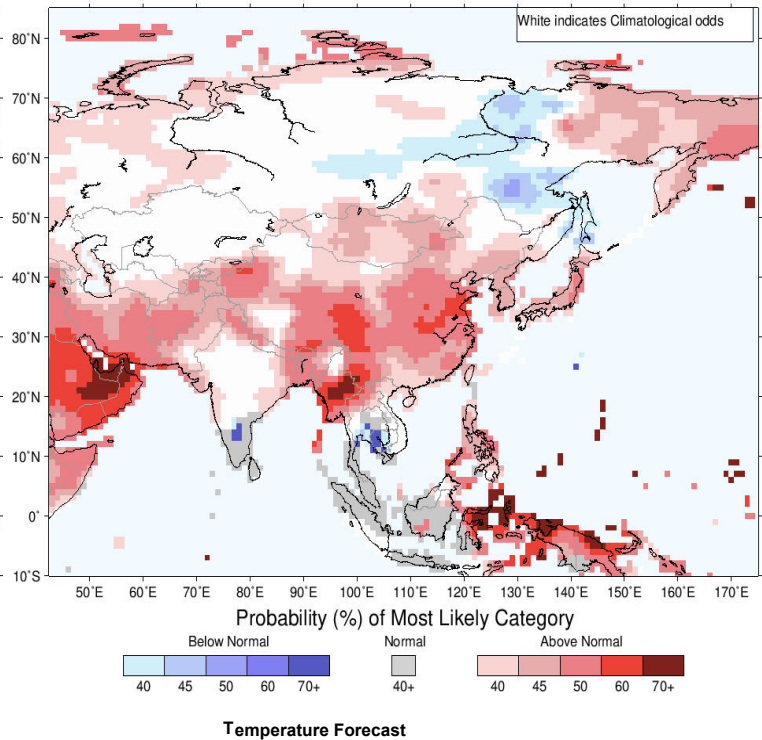
IRI Multi-Model Probability Forecast for Temperature for January–February–March 2023, Issued December 2022
