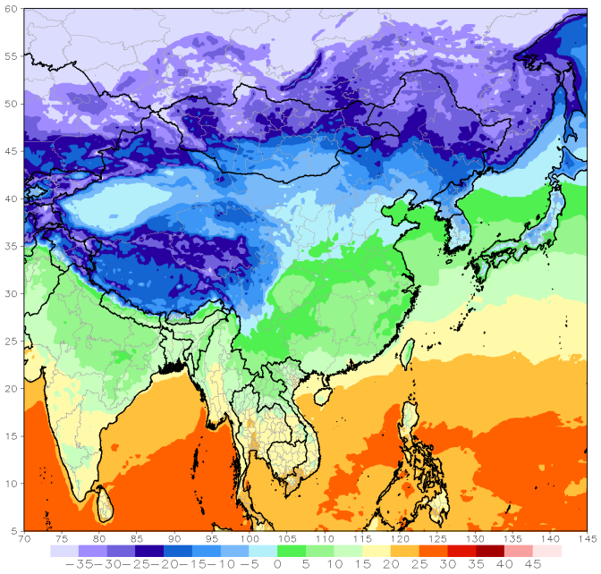
GFS week1 Temperature Min (C) Period: 18z06Jan2023 - 18z12Jan2023
