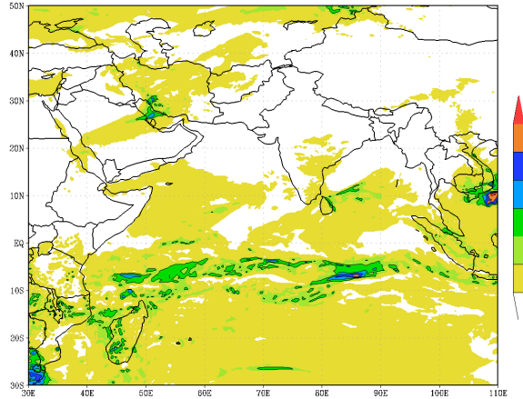
IMD :GFS MODEL(12 Km) RAINFALL (mm) FORECAST (24 HR) based on 00 UTC of 05-01-2023 valid for 03 UTC of 06-01-2023
