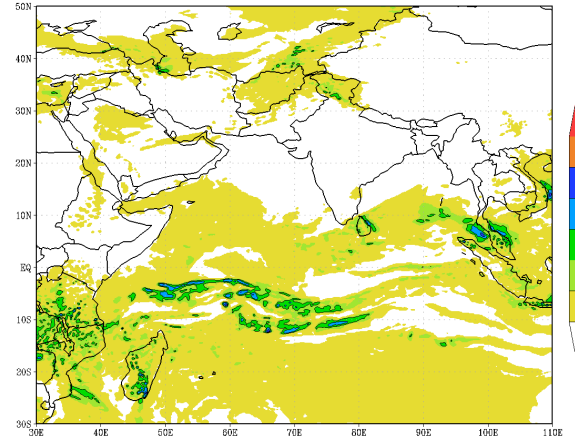
IMD :GFS MODEL(12 Km) RAINFALL (mm) FORECAST (96 HR) based on 00 UTC of 05-01-2023 valid for 03 UTC of 09-01-2023
