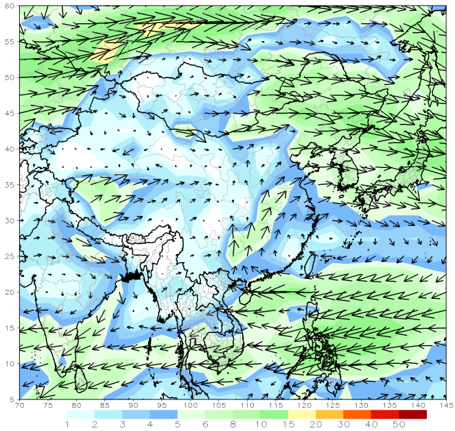
GFS 850mb week1 Mean Vector Wind Total (m/s) Period: 18z06Jan2023 - 18z12Jan2023
