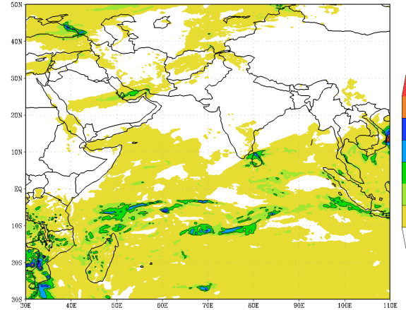
IMD :GFS MODEL(12 Km) RAINFALL (mm) FORECAST (48 HR) based on 00 UTC of 05-01-2023 valid for 03 UTC of 07-01-2023
