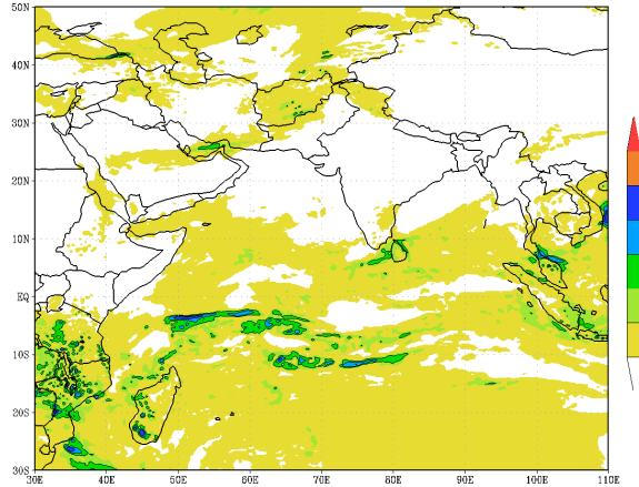
IMD :GFS MODEL(12 Km) RAINFALL (mm) FORECAST (72 HR) based on 00 UTC of 05-01-2023 valid for 03 UTC of 08-01-2023
