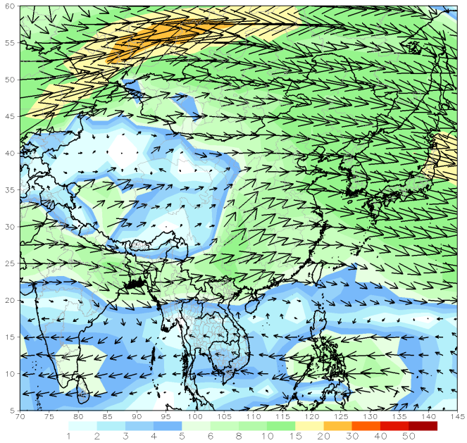
GFS 700mb week1 Mean Vector Wind Total (m/s) Period: 18z06Jan2023 - 18z12Jan2023
