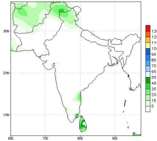
NCEP GFS Ensemble Forecast 1-7 Day Precipitation (mm) from: 05Jan2023 05Jan2023-11Jan2023 Accumulation
