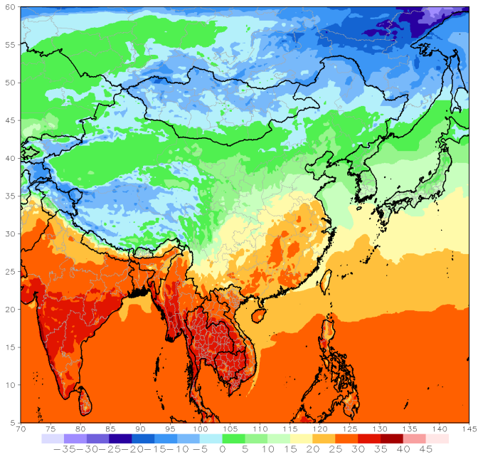
GFS week1 Temperature Max (C) Period: 18z06Jan2023 - 18z12Jan2023
