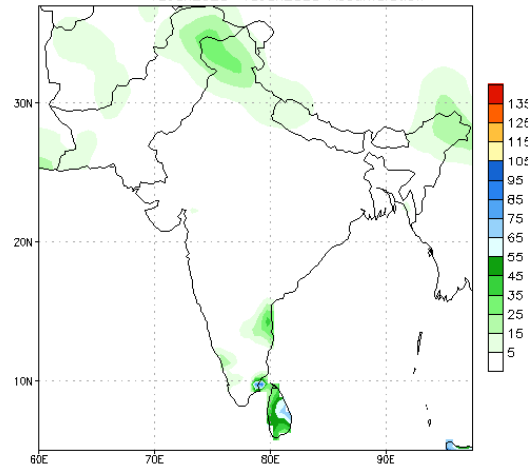
NCEP GFS Ensemble Forecast 8-14 Day Precipitation (mm) from: 05Jan2023 12Jan2023-18Jan2023 Accumulation
