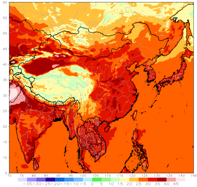
GFS week1 Temperature Max (C) Period: 18z18Aug2023 - 18z24Aug2023
