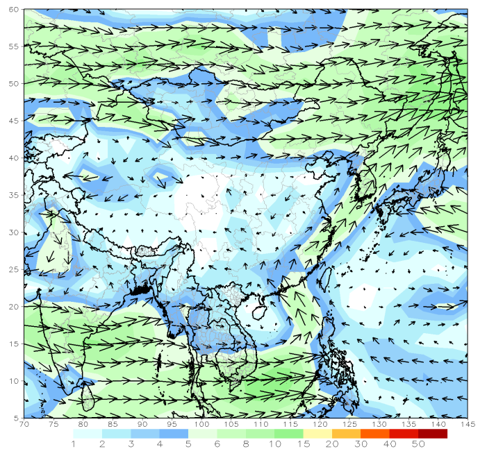
GFS 700mb week1 Mean Vector Wind Total (m/s) Period: 18z18Aug2023 - 18z24Aug2023
