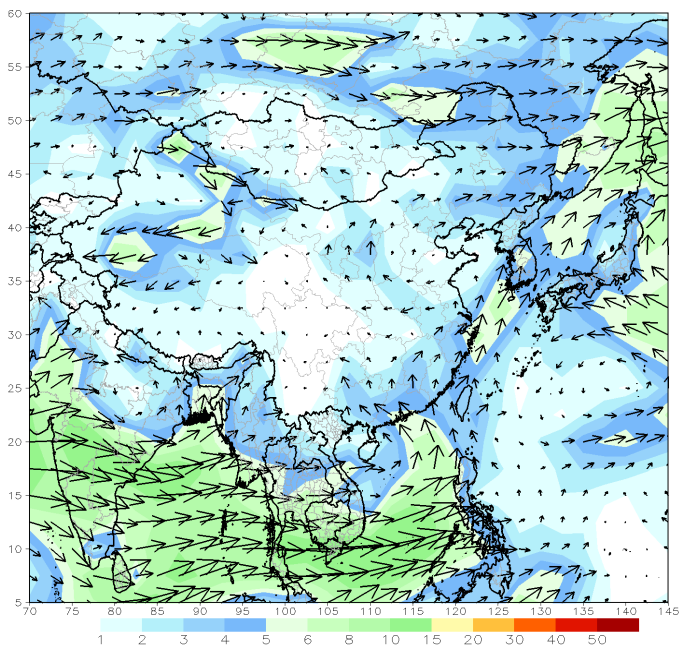
GFS 850mb week1 Mean Vector Wind Total (m/s) Period: 18z18Aug2023 - 18z24Aug2023
