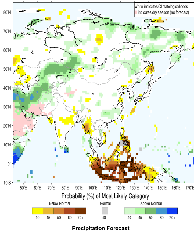
IRI Multi-Model Probability Forecast for Precipitation for September–October–November 2023, Issued August 2023
