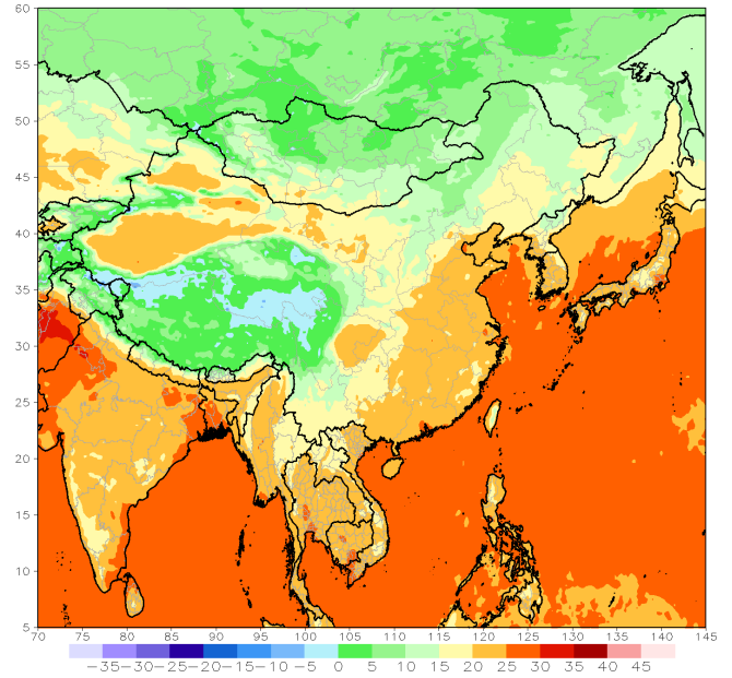
GFS week1 Temperature Min (C) Period: 18z18Aug2023 - 18z24Aug2023
