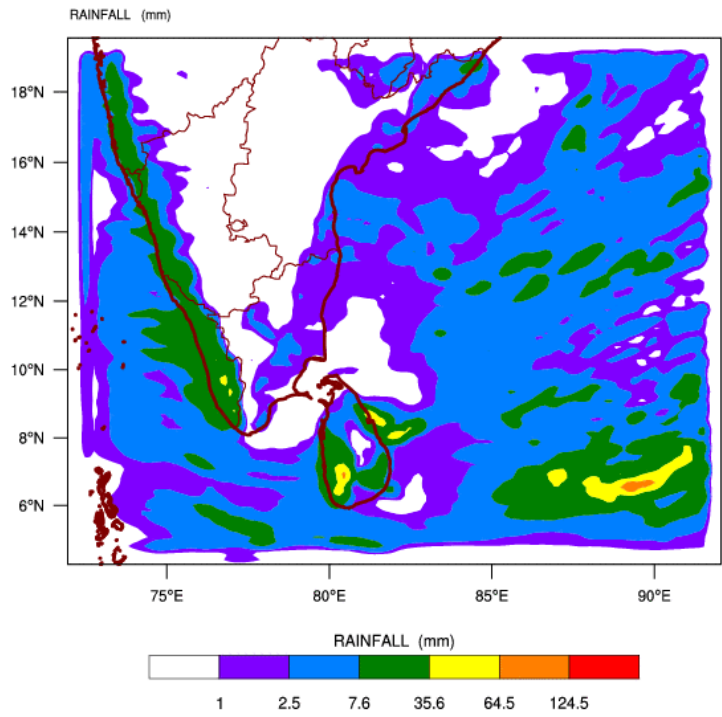
WRF MODEL FORECAST (48 HR.) RAINFALL(mm)\ based on 00 UTC of 21-08-2016 valid for 03 UTC of 23-08-2016
