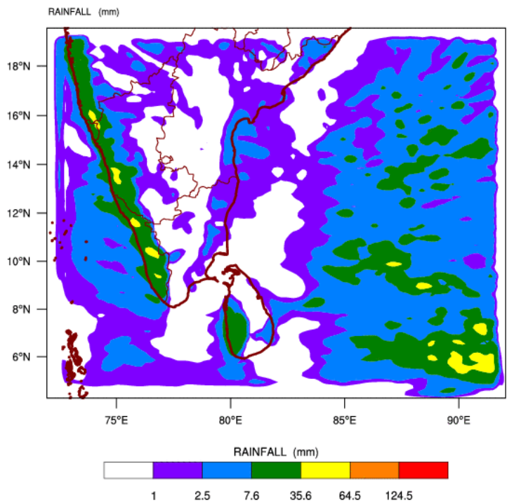
WRF MODEL FORECAST (72 HR.) RAINFALL(mm)\ based on 00 UTC of 21-08-2016 valid for 03 UTC of 24-08-2016
