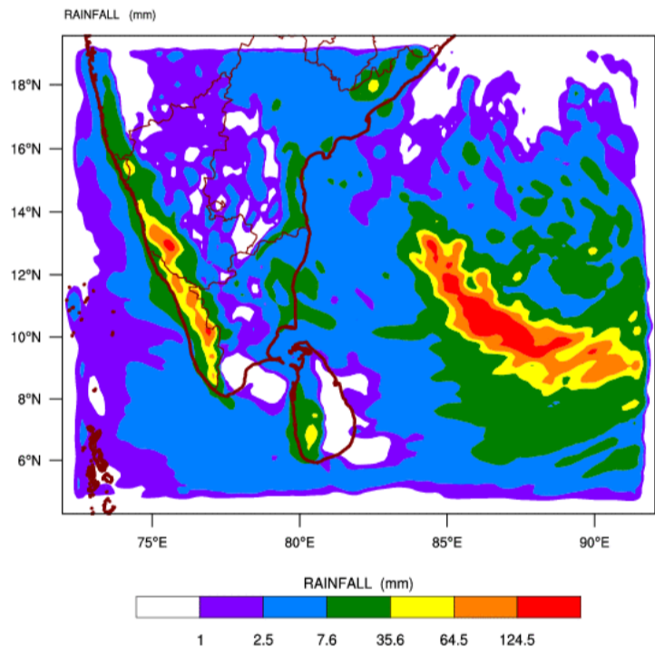
WRF MODEL FORECAST (72 HR.) RAINFALL(mm)\ based on 00 UTC of 20-06-2016 valid for 03 UTC of 23-06-2016
