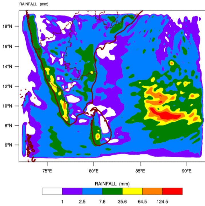
WRF MODEL FORECAST (48 HR.) RAINFALL(mm)\ based on 00 UTC of 20-06-2016 valid for 03 UTC of 22-06-2016
