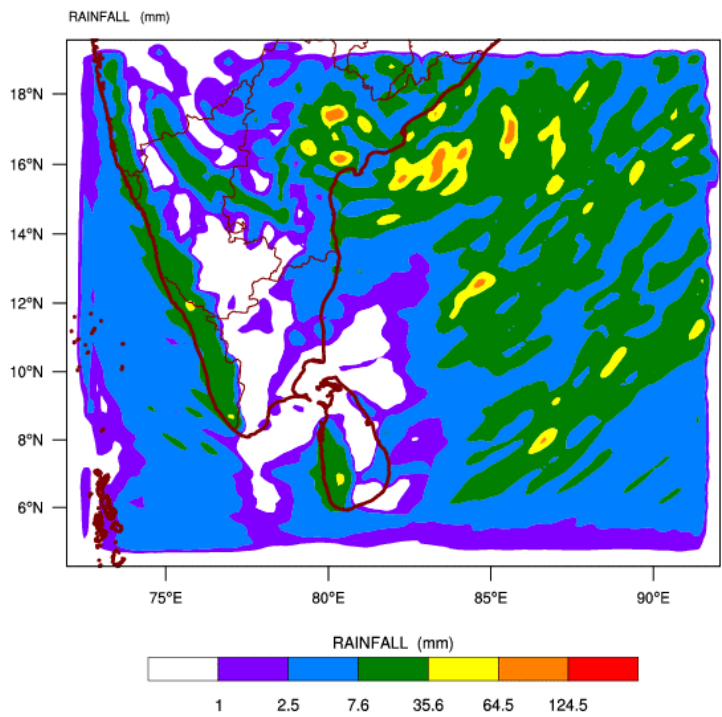
WRF MODEL FORECAST (72 HR.) RAINFALL(mm)\ based on 00 UTC of 12-09-2016 valid for 03 UTC of 15-09-2016
