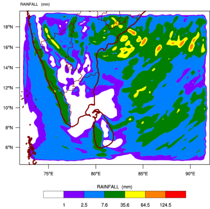
WRF MODEL FORECAST (48 HR.) RAINFALL(mm)\ based on 00 UTC of 12-09-2016 valid for 03 UTC of 14-09-2016
